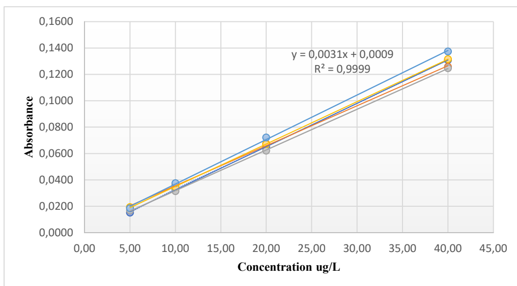
Figure 2. Linearity of the lead calibration curve.
