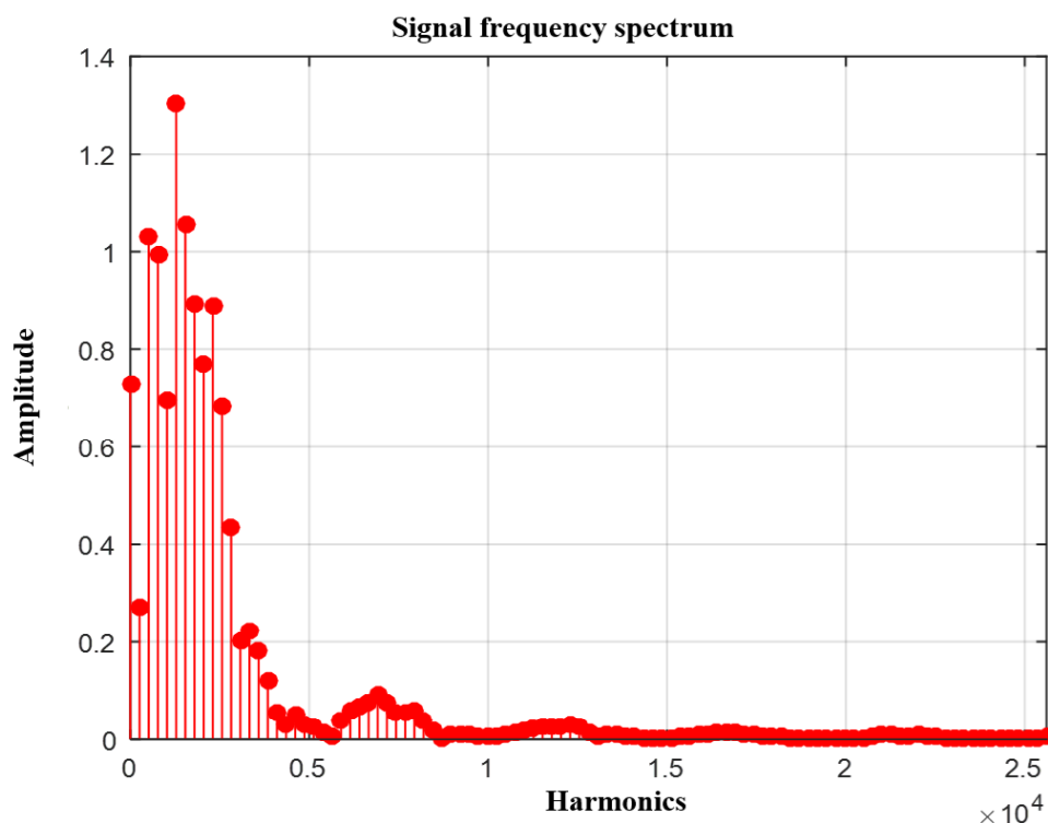
Figure 7. The frequency spectrum of the signal at month 40 using harmonics and its amplitude.
